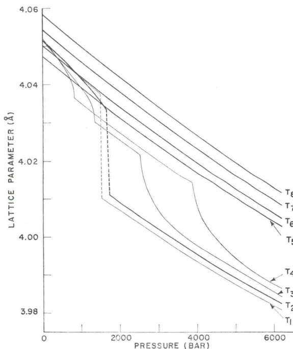
FIG. 2. Variation of the lattice parameter with pressure. Heavy curves at 200^\circ , 240^\circ , 255^\circ , 275^\circ , and 295^\circ\text{K} are accurately known, whereas the three lighter curves are less well established (see text). Lattice parameters in the tetragonal phase (low-pressure portions of the 190^\circ and 220^\circ\text{K} curves) represent the cube root of the unit-cell volume. T_1=190^\circ\text{K} , T_2=200^\circ\text{K} , T_3=210^\circ\text{K} , T_4=220^\circ\text{K} , T_5=240^\circ\text{K} , T_6=255^\circ\text{K} , T_7=275^\circ\text{K} , T_8=295^\circ\text{K} .
